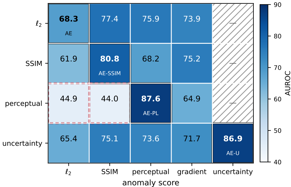
training objective
